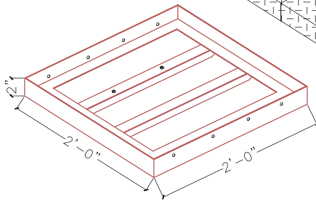
ALUMINUM FRAME DRAIN BOX
