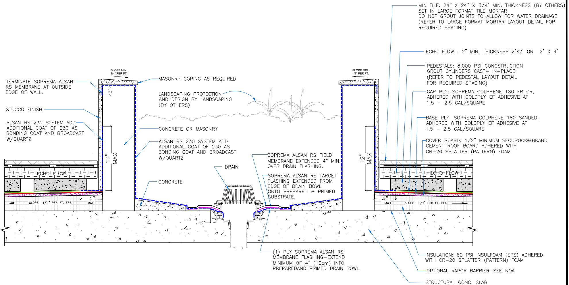
PLANTER FLASHING DETAIL (-465 PSF NAO)
