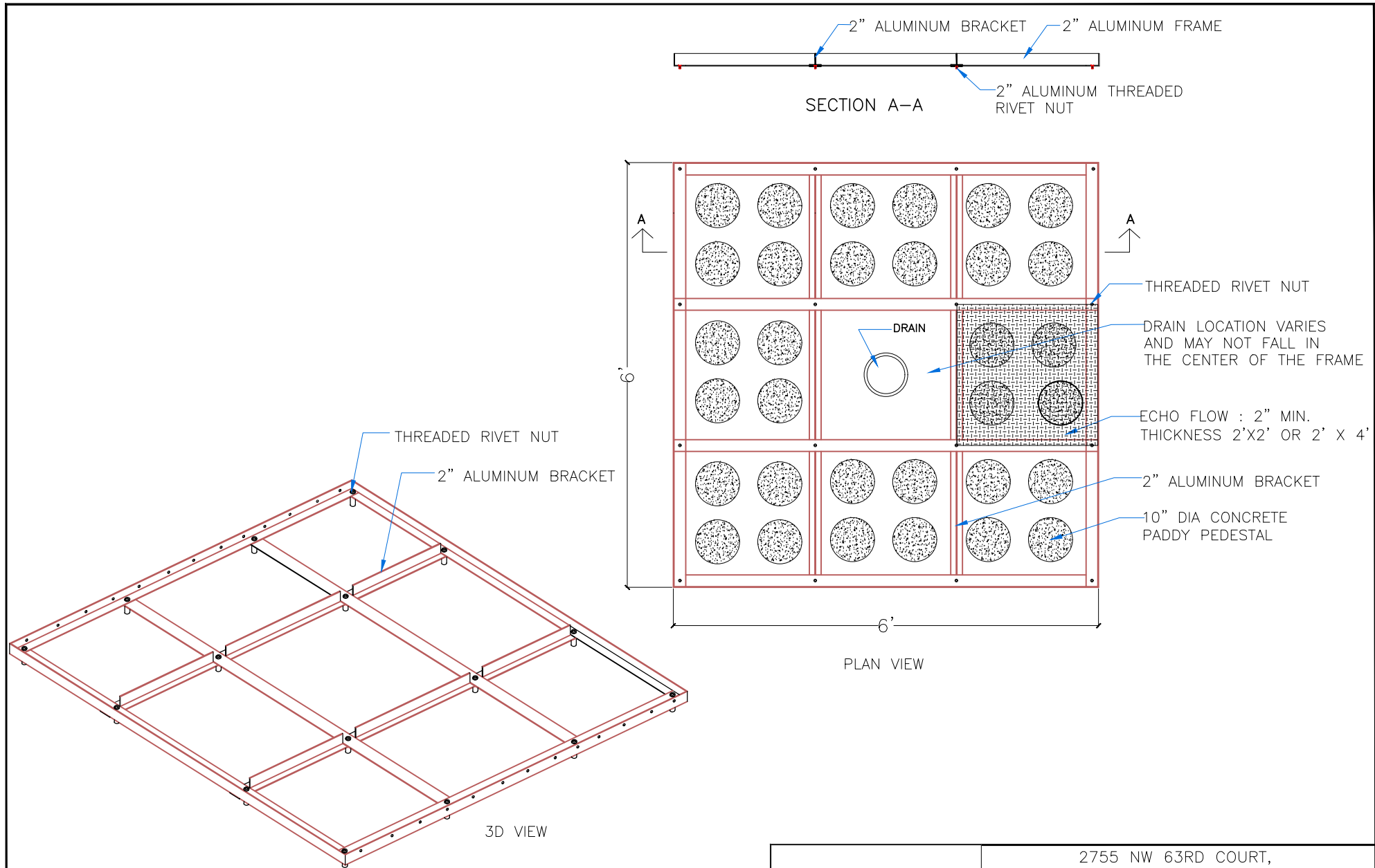
6' X 6' TILE ALUMINUM FRAME DRAIN BOX DETAIL
